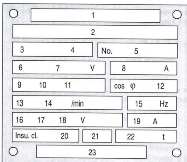
Fig. 1.10.1 Rating plate
